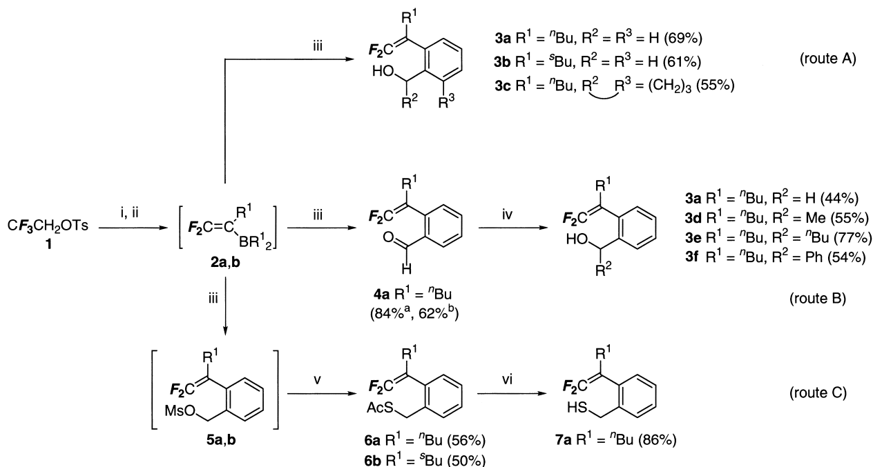
Scheme 1. Preparation of \beta,\beta -difluorostyrenes functionalized at the ortho position.
