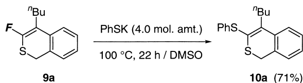
Scheme 2. Introduction of substituent at the 3-position.
